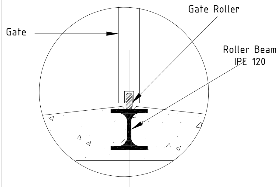
DETAIL -A
