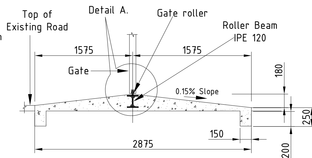
SECTION C-C
