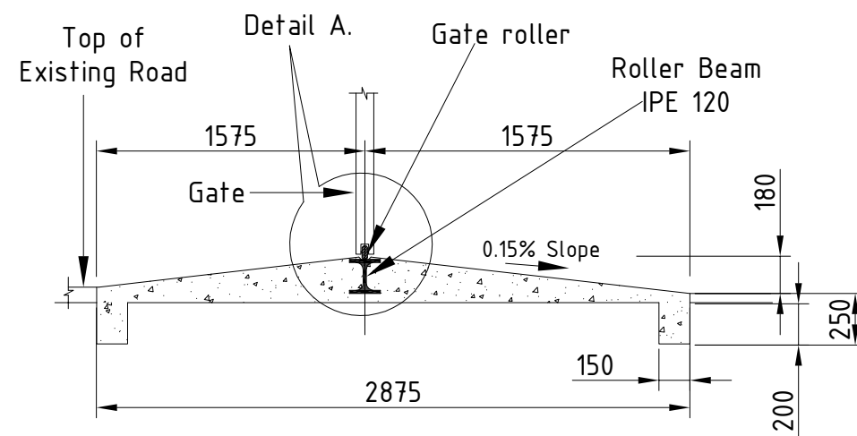
SECTION C-C
